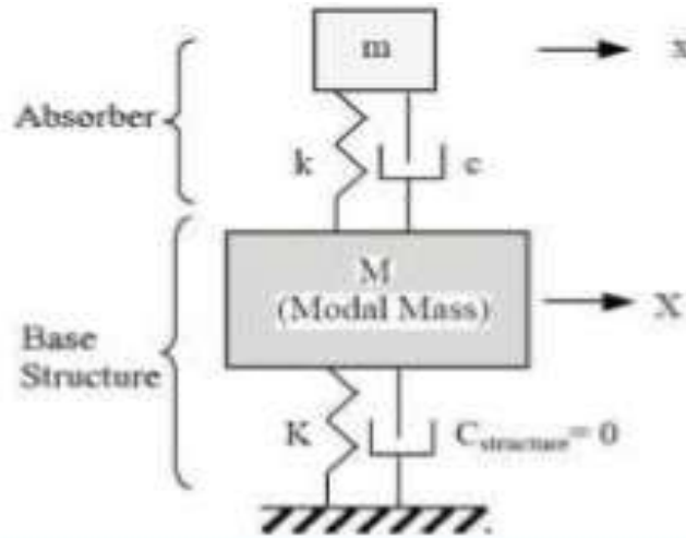
Fig: 3.1 A schematic representation of damped vibration absorber suggested by Den Hartog
