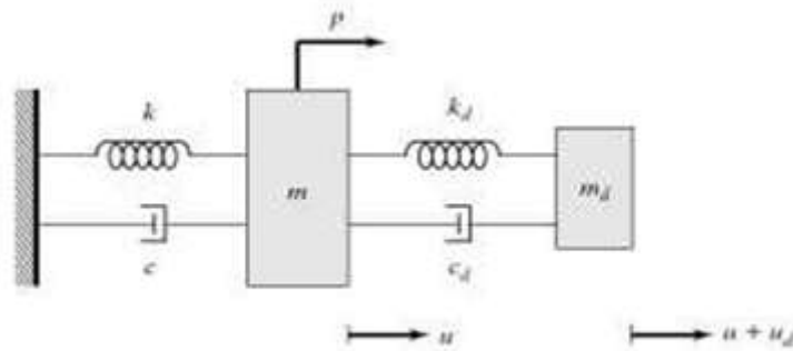
Fig. 3.4: SDOF-TMD system
