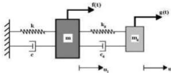
Fig: Model of SDOF structure and TMD
