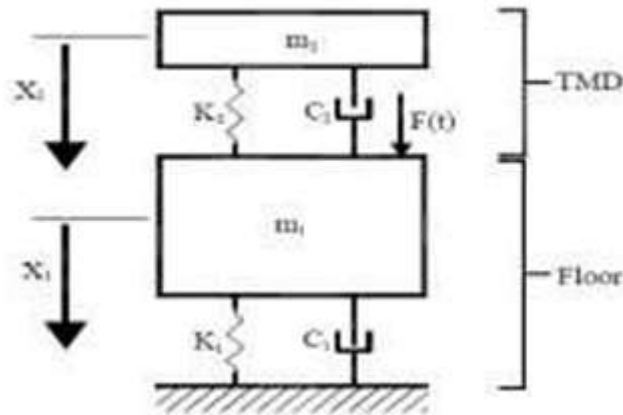
Fig. 3.3: Schematic Representation of a Two DOF System
